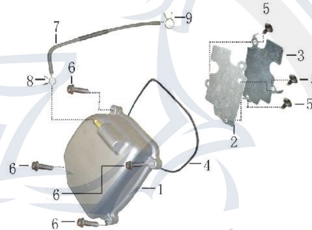
Ventildeckel GY6-2
