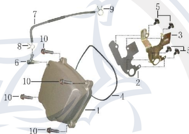
Ventildeckel GY6-1
