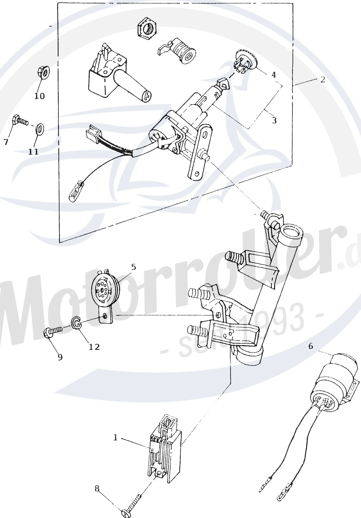
FIG.25 ELECTRICAL EQUIPMENT, KEY SET
