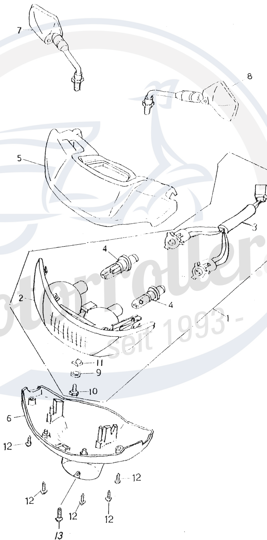
FIG.21 HEAD LIGHT, BACK VIEW MIRROR
