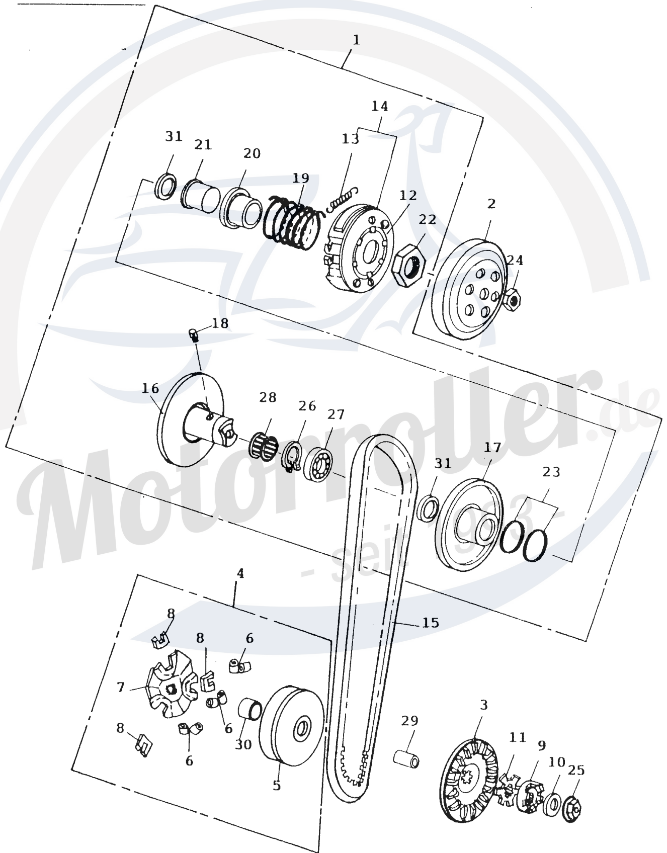
FIG.10 CLUTCH
