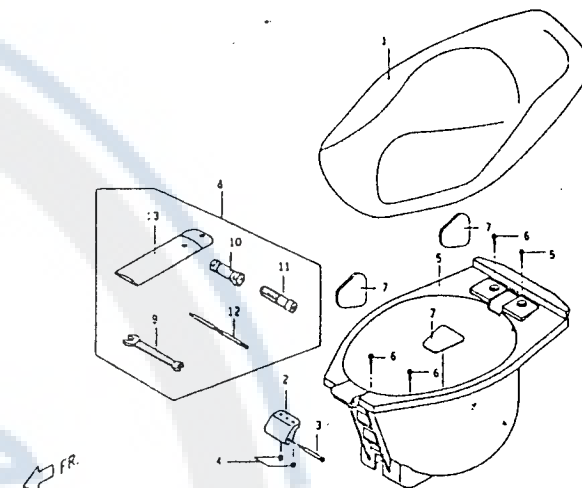
F9 座墊, 置物箱, 工具箱 SEAT HELMET CASE TOOL KIT
