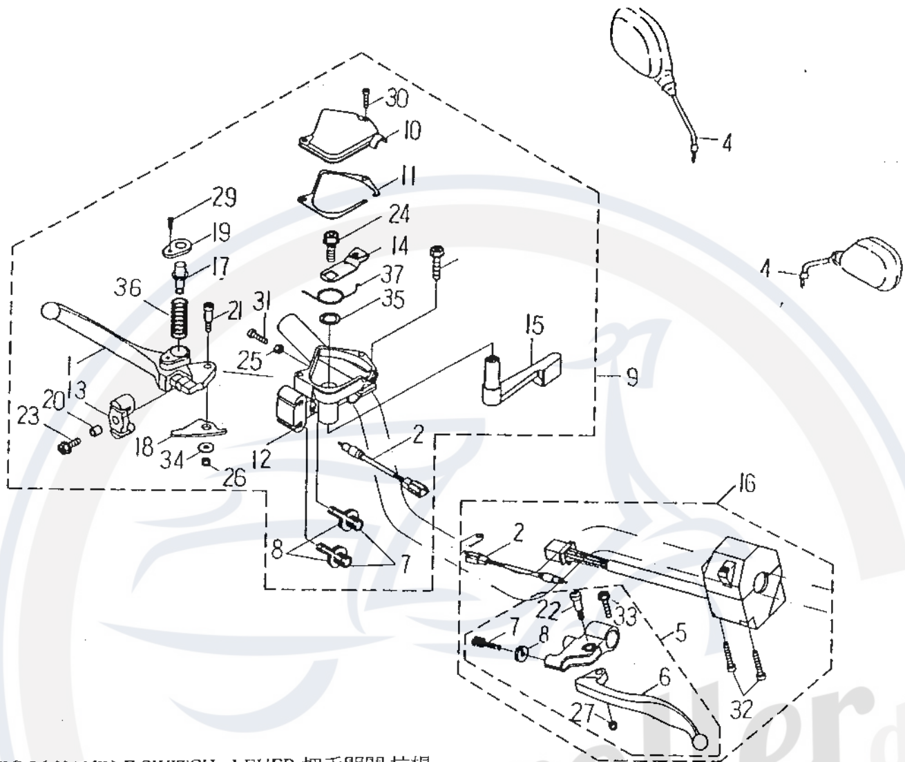
FIG.26 HANDLE SWITCH , LEVER 把手開關,拉桿
