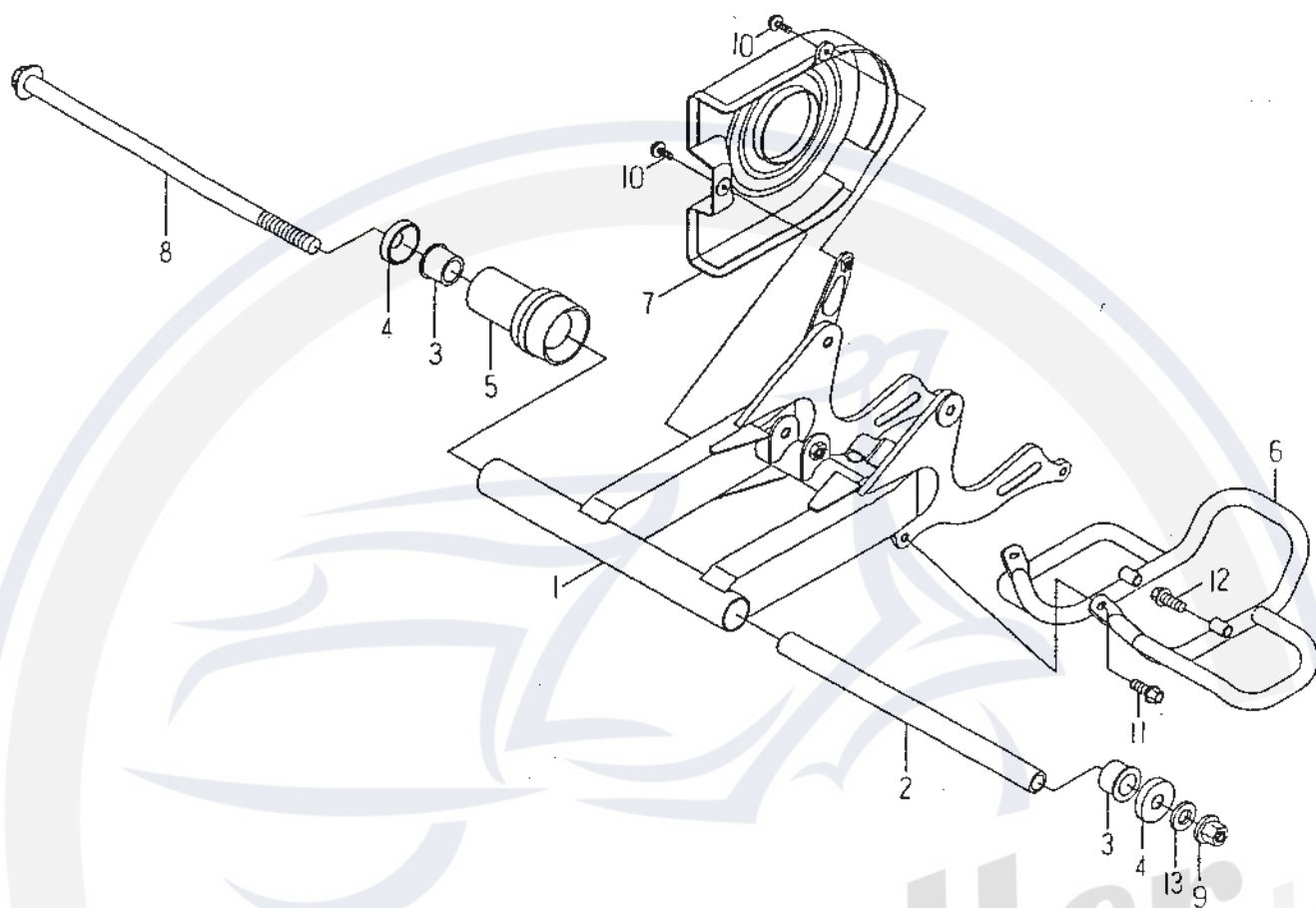
FIG. 14 REAR ARM 擺動臂
