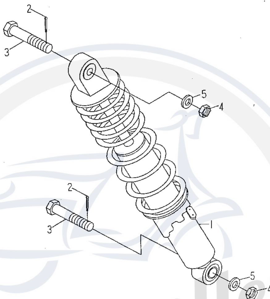
FIG.15 REAR SUSPENSION 後懸吊系統
